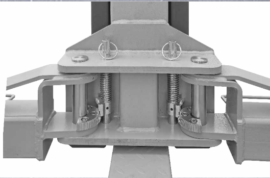
AUTOMATIC ARM LOCK
